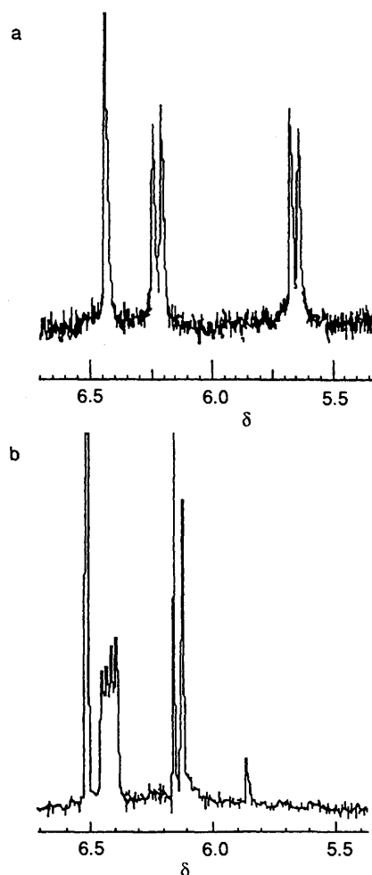
Fig. 1. ^1\text{H} NMR spectra (a) compound 9 and (b) compound 17 , showing the inversion of configuration at C-4'.
